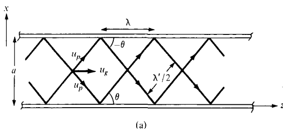
Figure 12.10 (a) Decomposition of TE_{10} mode into two plane waves; (b) relationship between u' , u_p , and u_g .
